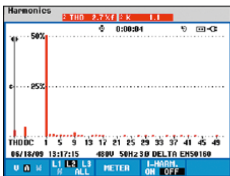
Harmonic current spectrum with filter. THD: 2.7%
