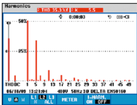
Harmonic current spectrum without filter. THD: 35.3%
